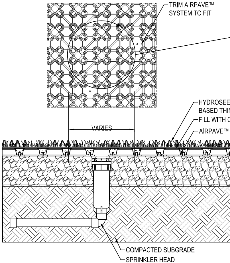
DETAIL A
