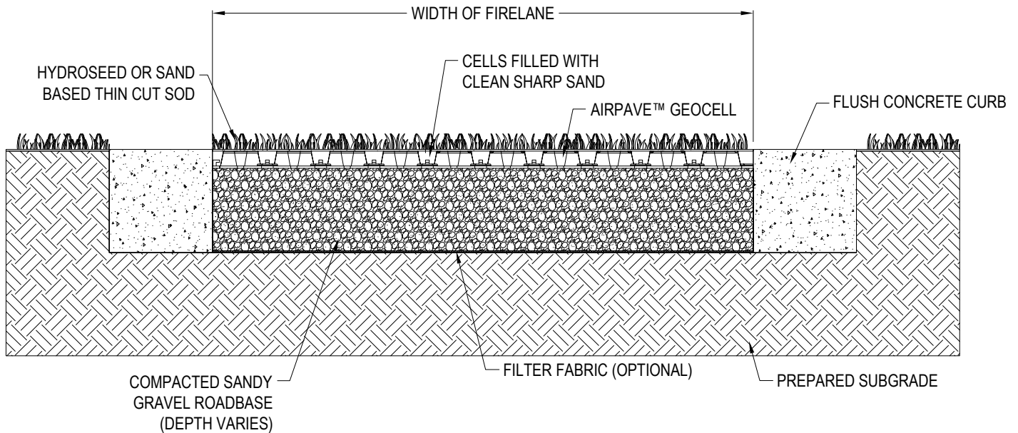
SECTION AT RAISED CURB
