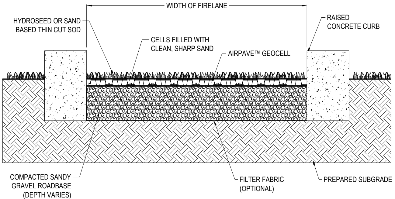
SECTION AT RAISED CURB
